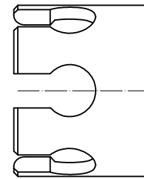
BAR PULL GRIPPERS PBG0812-PBG1250 & PBG21MM-PBG32MM
